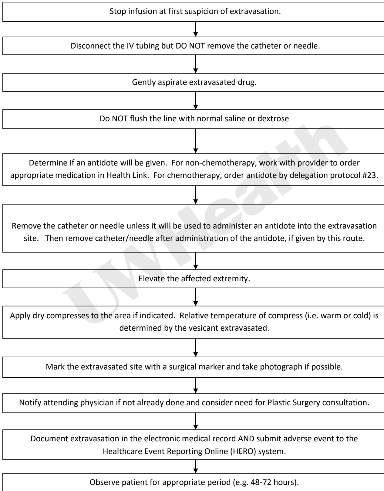
Figure 1. Workflow algorithm
